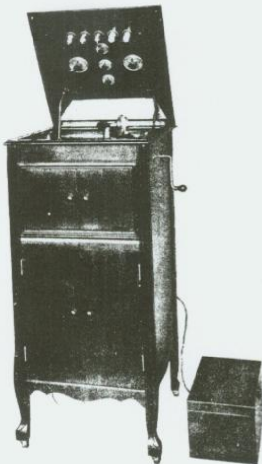
FIG. 1—RADIO LA IX INSTALLED IN STANDARD PHONOGRAPH
