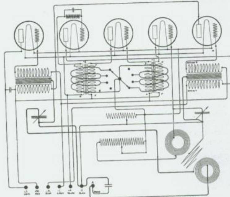
FIG. 6 - SCHEMATIC WIRING DIAGRAM OF RADIOLA IX
