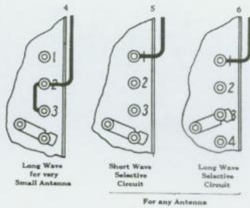
Fig. 3—Showing Antenna Connections to Different Binding Posts
