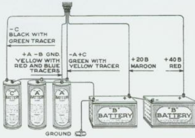
Fig. 2—Battery Connections
