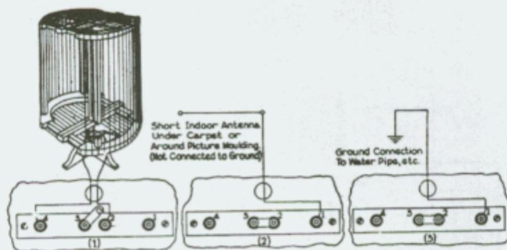
Fig. 5. Connection of Exterior Loop, Indoor Antenna, etc.
