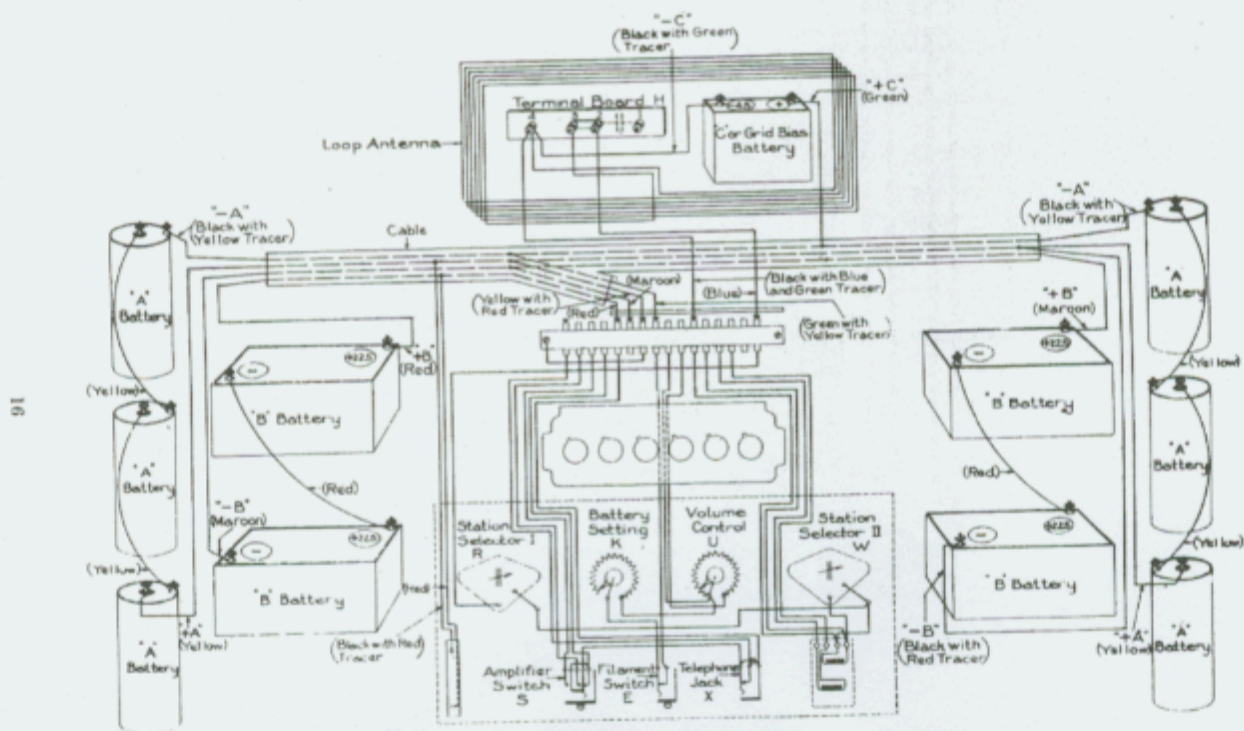
Fig. 6. Connection Diagram of Radiola Super-Heterodyne
