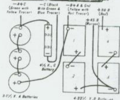
Diagram of Battery Connections for Portable Unit
