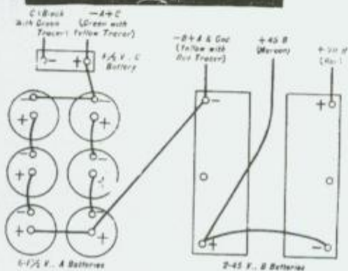
Diagram of Battery Connections When Using Home Battery Box
