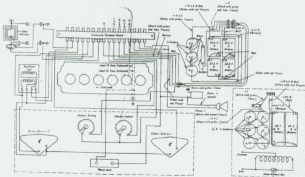
Diagram of Battery Connections When Using Home Battery Box
