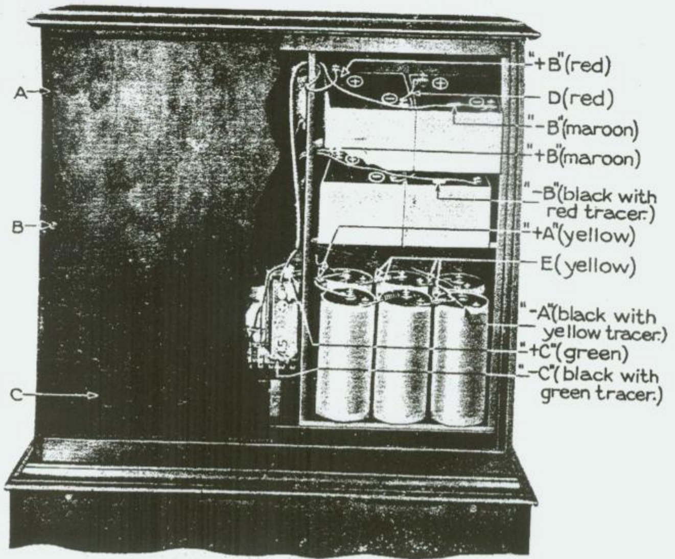
Fig. 1. Rear View, Showing Battery Connections
