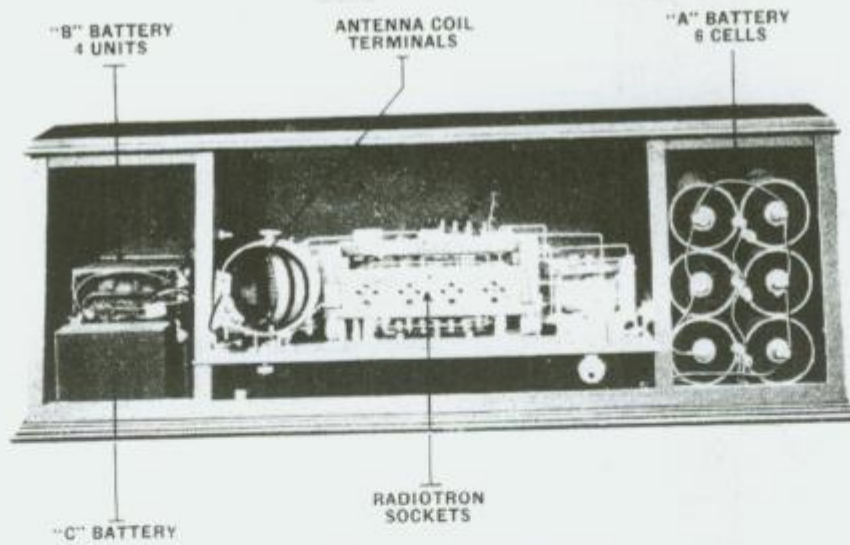
Fig. 5 Internal View of Radiola Regenflex
