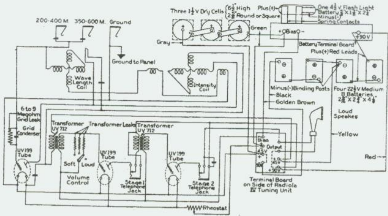
Fig. 5. Schematic Wiring Diagram of Radiola IV
