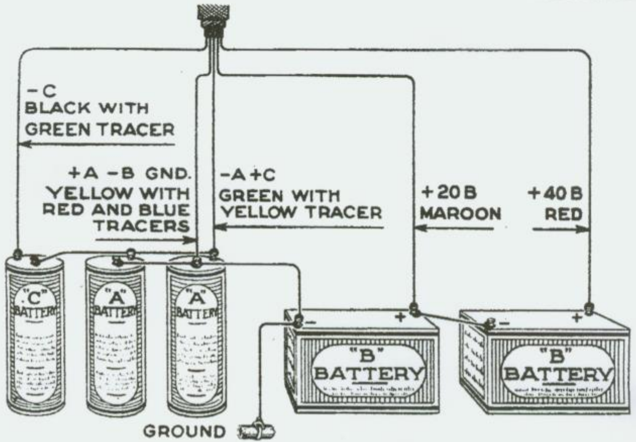
Fig. 2—Battery Connections
