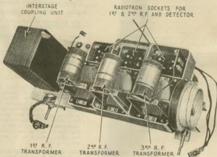
Figure 4—View of receiver with shields removed
