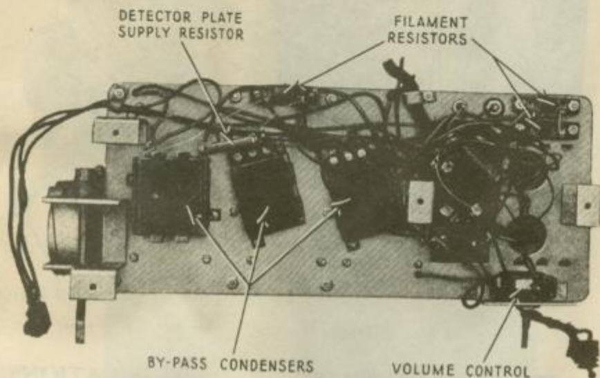
Figure 3—Sub-chassis view of receiver
